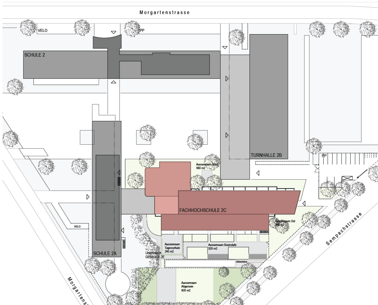
Situationsplan
