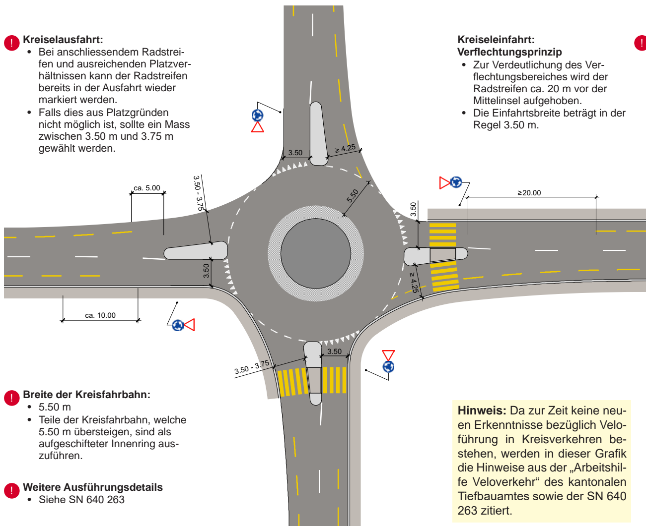
Situationsplan (1:500)
