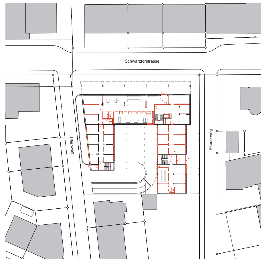
Situation/Erdgeschoss
